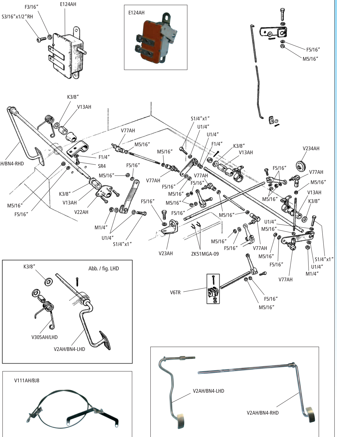
Abb. RHD / fig. RHD illustrated – Twin Carb BN4, BN6, BN7, BT7
