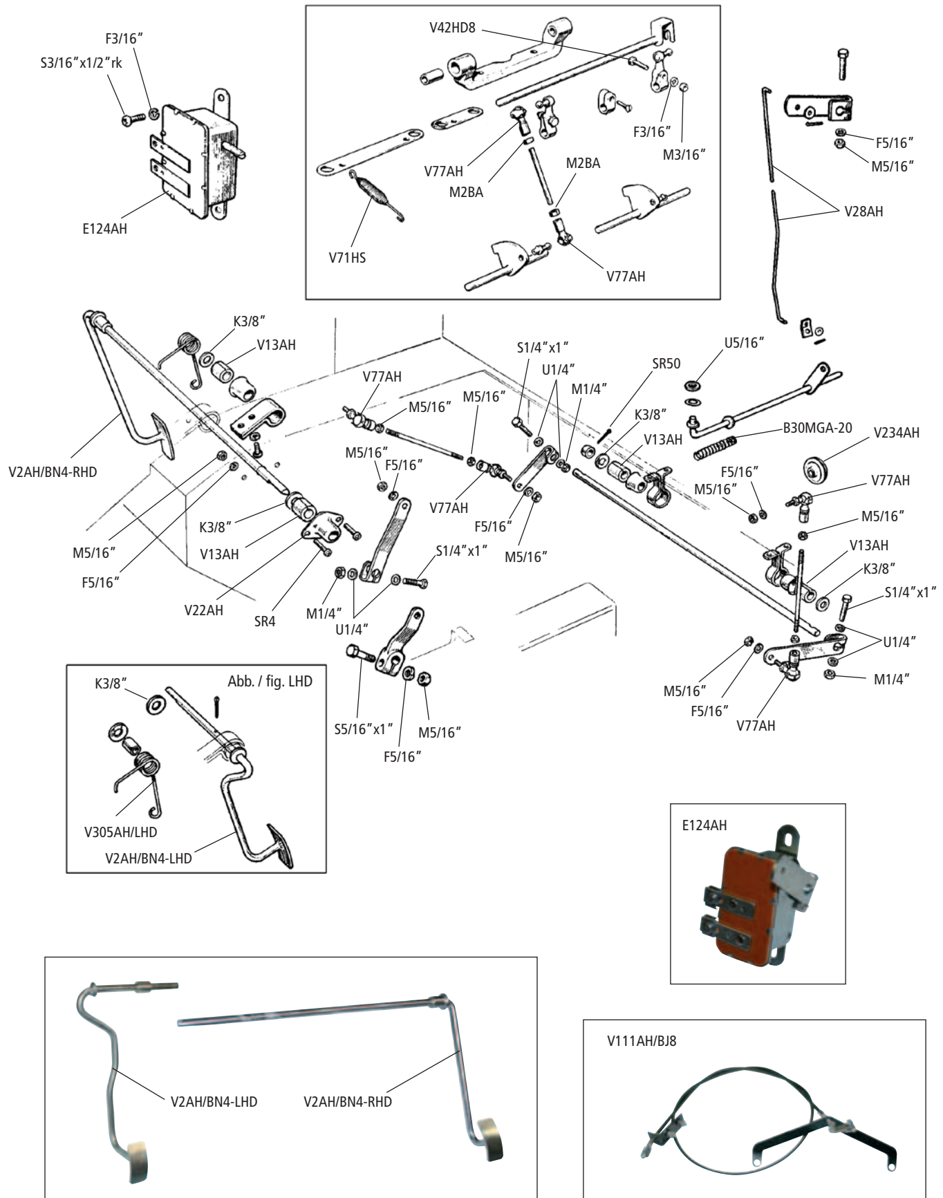
Abb. RHD / fig. RHD illustrated – Tri Carb BN7, BT7
